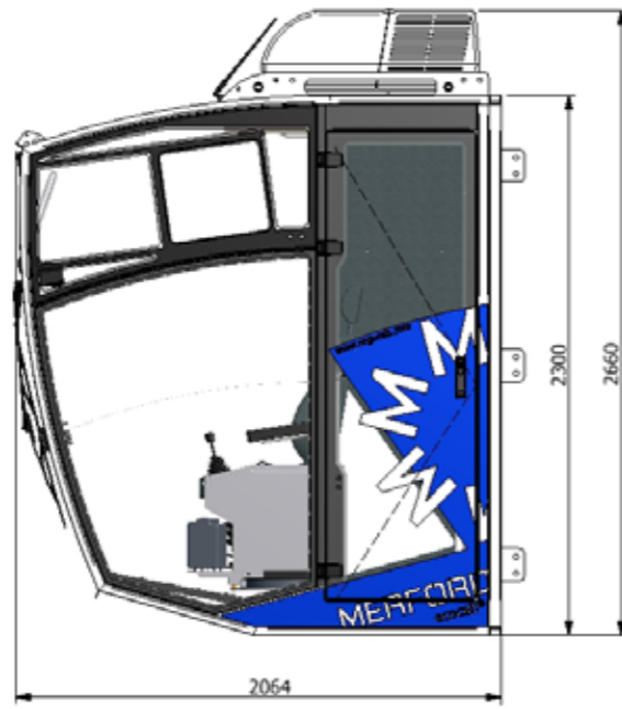
LEFT OUTSIDE VIEW
